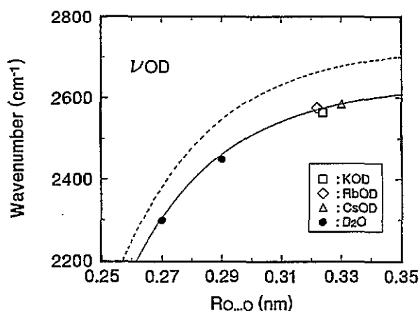
Figure 17. Frequency-distance diagram for a linear O—D \cdots O system with ambient-pressure data for KOD, RbOD and CsOD. The broken curve represents the empirical correlation of Mikenda [22], the D 2 O data are results of high-pressure Raman measurements on ice [24].
