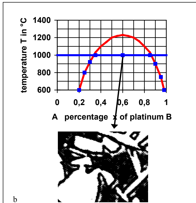
Fig. 2 a. Phase diagram of gold platinum alloys (Au Pt): At 1000^\circ\text{C} gold may solve up to 35 % Pt. A higher percentage, 60 % Pt will lead to segregation into the two phases \alpha and \beta , fig. 2 b. The \alpha -phase contains 35 % Pt, the \beta -phase contains 85 % Pt.
